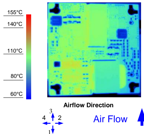
Figure 8. Thermal Image for Airflow Direction 3 (4.5A output, 55°C ambient, 200 LFM, typical Vin, open frame, unit soldered onto a fixture board)
